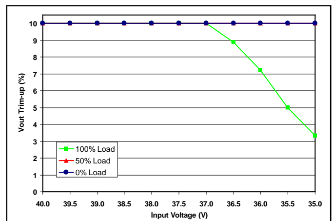
Figure 24: Achievable trim-up percentage vs. input voltage at output loads of 0%, 50% and full load.
