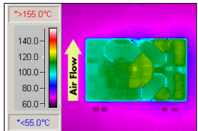
Figure 12: Thermal plot of converter at 60 amp load with 55°C air flowing from pin 3 to pin 1 at the rate of 200 LFM with nominal Vin and 4 output pins. Test board is 4oz., 6 layer. Converter PCB is 6oz., 12 layer.
