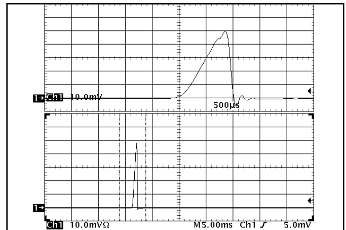
Figure 22: Load current (20A/div) as a function of time when the converter attempts to turn on into a 1 \text{ m}\Omega short circuit. Bottom trace (5 ms/div) is an expansion of the on-time portion of the top trace.
