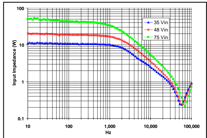
Figure 28: Magnitude of incremental input impedance ( Z_{in} = v_{in}/i_{in} ) for minimum, nominal, and maximum input voltage at full rated power.
