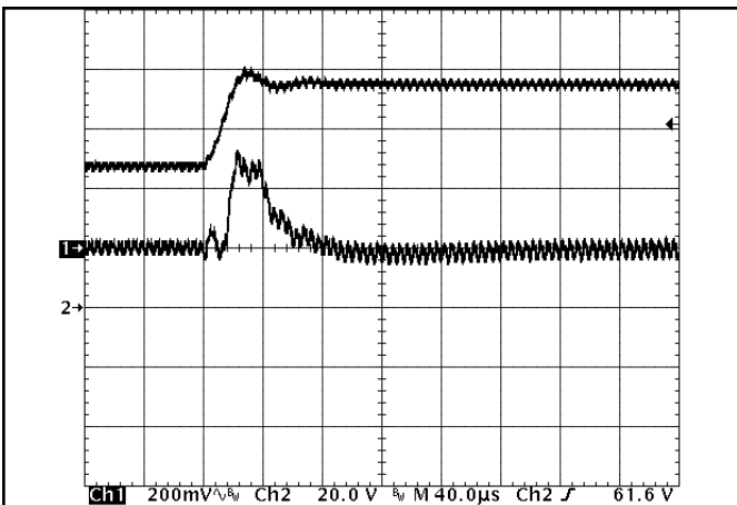
Figure 21: Output voltage response to step-change in input voltage (50V to 100V in 40 \mu\text{s} ). Load cap: 10 \mu\text{F} , 100 \text{ m}\Omega ESR tantalum capacitor and 1 \mu\text{F} ceramic cap. Ch 1: V_{\text{out}} (200 mV/div), Ch 2: V_{\text{in}} (20V/div).
