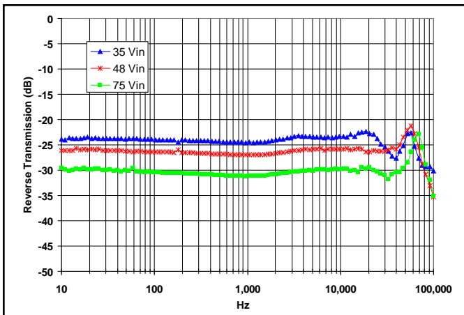
Figure 27: Magnitude of incremental reverse transmission ( RT = i_{in}/i_{out} ) for minimum, nominal, and maximum input voltage at full rated power.
