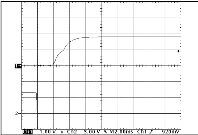
Figure 13: Turn-on transient at full rated load (resistive load) (2 ms/div) Input voltage pre-applied. Ch 1: V_{out} (1V/div). Ch 2: ON/OFF input (5V/div)
