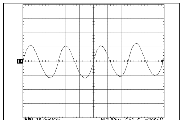
Figure 18: Input Terminal Ripple Current, i_c , at full rated output current and nominal input voltage with 10µH source impedance and 47µF electrolytic capacitor (200 mA/div). See Figure 17.
