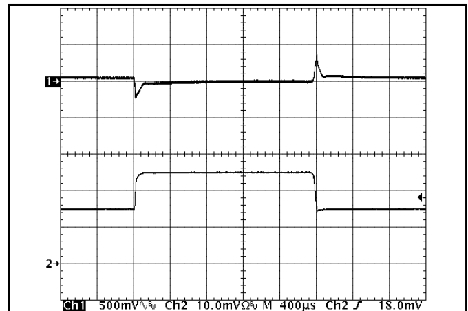
Figure 16: Output voltage response to step-change in load current (50%-75%-50% of I_{out(max)} ; di/dt = 1A/\mu s ). Load cap: 470µF, 30 mΩ ESR tantalum cap and 1µF ceramic cap. Ch 1: V_{out} (500mV/div), Ch 2: I_{out} (20A/div).
