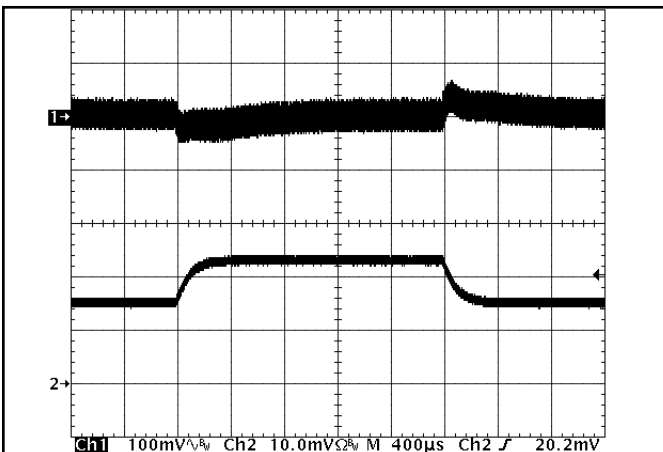
Figure 15: Output voltage response to step-change in load current (50%-75%-50% of I_{out(max)} ; di/dt = 0.1A/\mu s ). Load cap: 10µF, 100 mΩ ESR tantalum cap and 1µF ceramic cap. Ch 1: V_{out} (100mV/div), Ch 2: I_{out} (20A/div).
