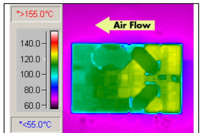
Figure 6: Thermal plot of converter at 56 amp load with 55°C air flowing from output to input at the rate of 200 LFM with nominal Vin and 2 output pins. Test board is 4oz., 6 layer. Converter PCB is 6oz., 12 layer.
