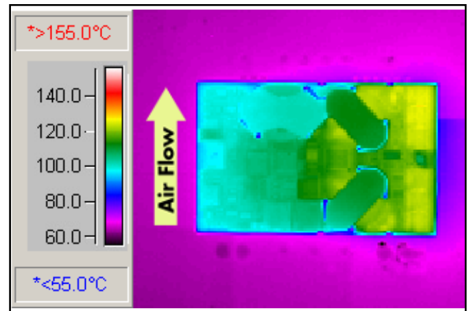
Figure 8: Thermal plot of converter at 55 amp load with 55°C air flowing from pin 3 to pin 1 at the rate of 200 LFM with nominal Vin and 2 output pins. Test board is 4oz., 6 layer. Converter PCB is 6oz., 12 layer.
