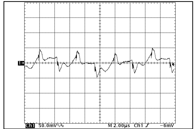
Figure 20: Output voltage ripple at nominal input voltage and rated load current (50 mV/div). Load capacitance: 1 \mu\text{F} ceramic capacitor and 15 \mu\text{F} tantalum capacitor. Bandwidth: 500 MHz. See Figure 17.
