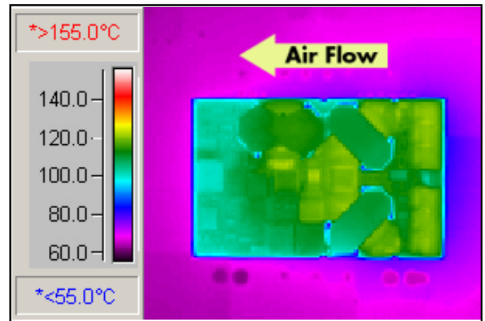
Figure 10: Thermal plot of converter at 60 amp load with 55°C air flowing from output to input at the rate of 200 LFM with nominal Vin and 4 output pins. Test board is 4oz., 6 layer. Converter PCB is 6oz., 12 layer.
