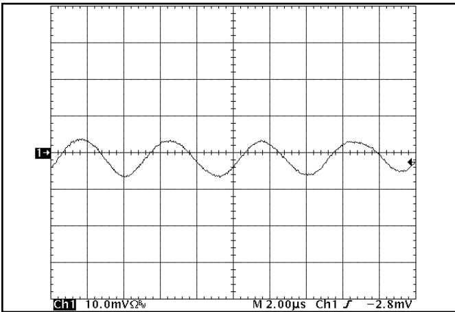
Figure 19: Input reflected ripple current, i_r , through a 10 \mu\text{H} source inductor at nominal input voltage and rated load current (10 mA/div). See Figure 17.
