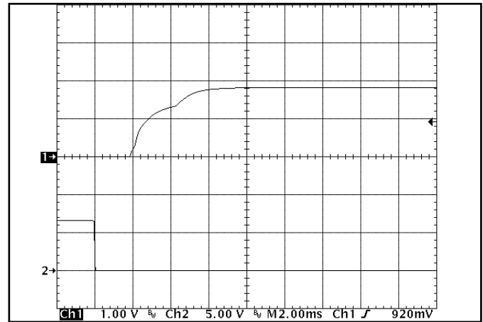
Figure 14: Turn-on transient at zero load current (2 ms/div). Ch 1: V_{out} (1V/div) Ch 2: ON/OFF input (5V/div)
