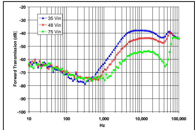
Figure 26: Magnitude of incremental forward transmission ( FT = v_{out}/v_{in} ) for minimum, nominal, and maximum input voltage at full rated power.
